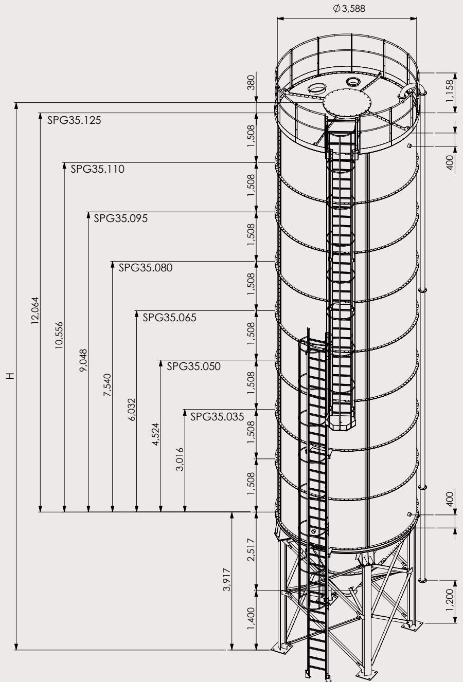
Overall Dimensions
