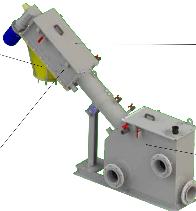
Polymer Outlet with Compacting Washing System
